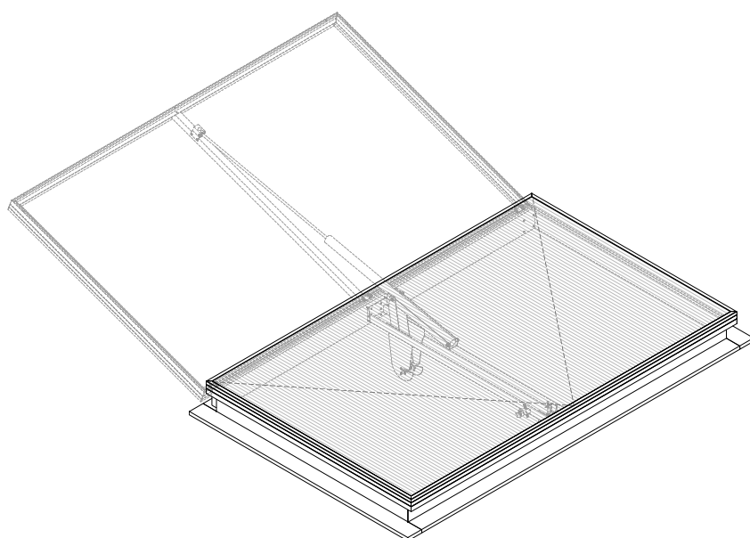
PERSPECTIVE VIEW OPENING SYSTEM
