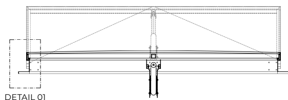
SECTION S2
